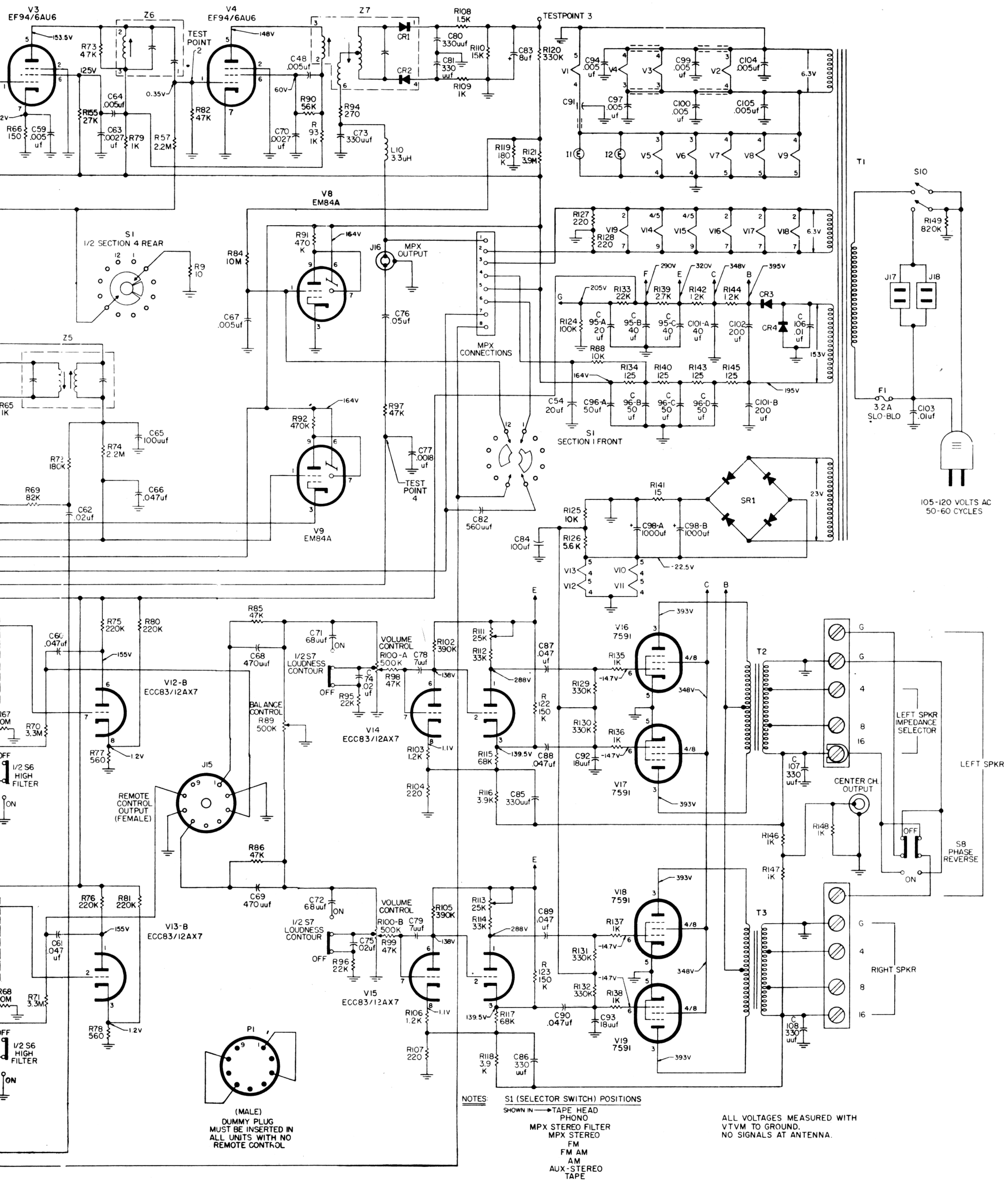
FISHER MODEL 800-B (SERIAL # 10001 TO 19999W/X/Y/Z) AM-FM STEREO RECEIVER
