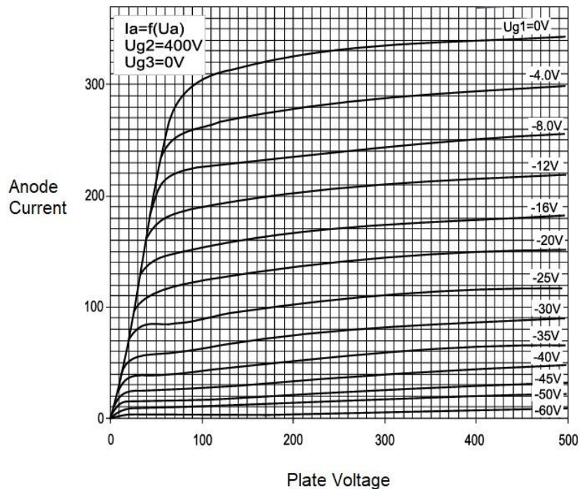
Plate Characteristics
