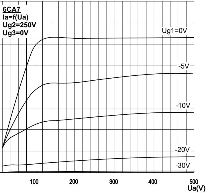
PLATE CHARACTERISTICS
