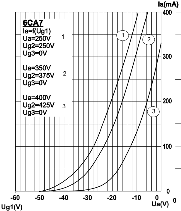
TRANSFER CHARACTERISTICS
